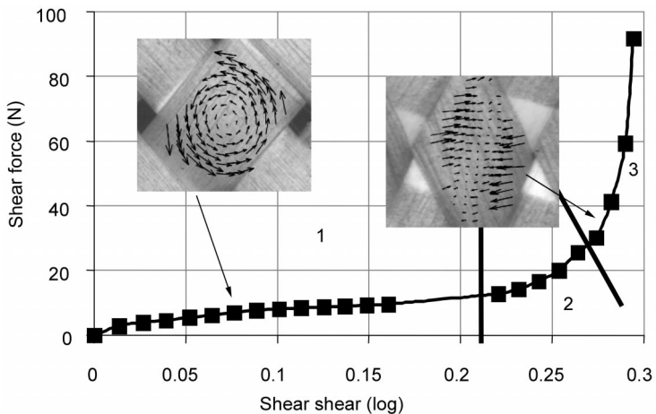
3.16 Shear curve and optical analysis (Dumont, 2003).
