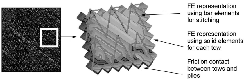
3.11 A 'representative cell' of the meso-mechanical model for NCF (Pickett et al. , 2005).
