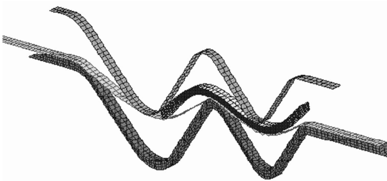
3.21 Forming of a Z reinforcement. Forming stage (Cheruet et al. , 2002).
